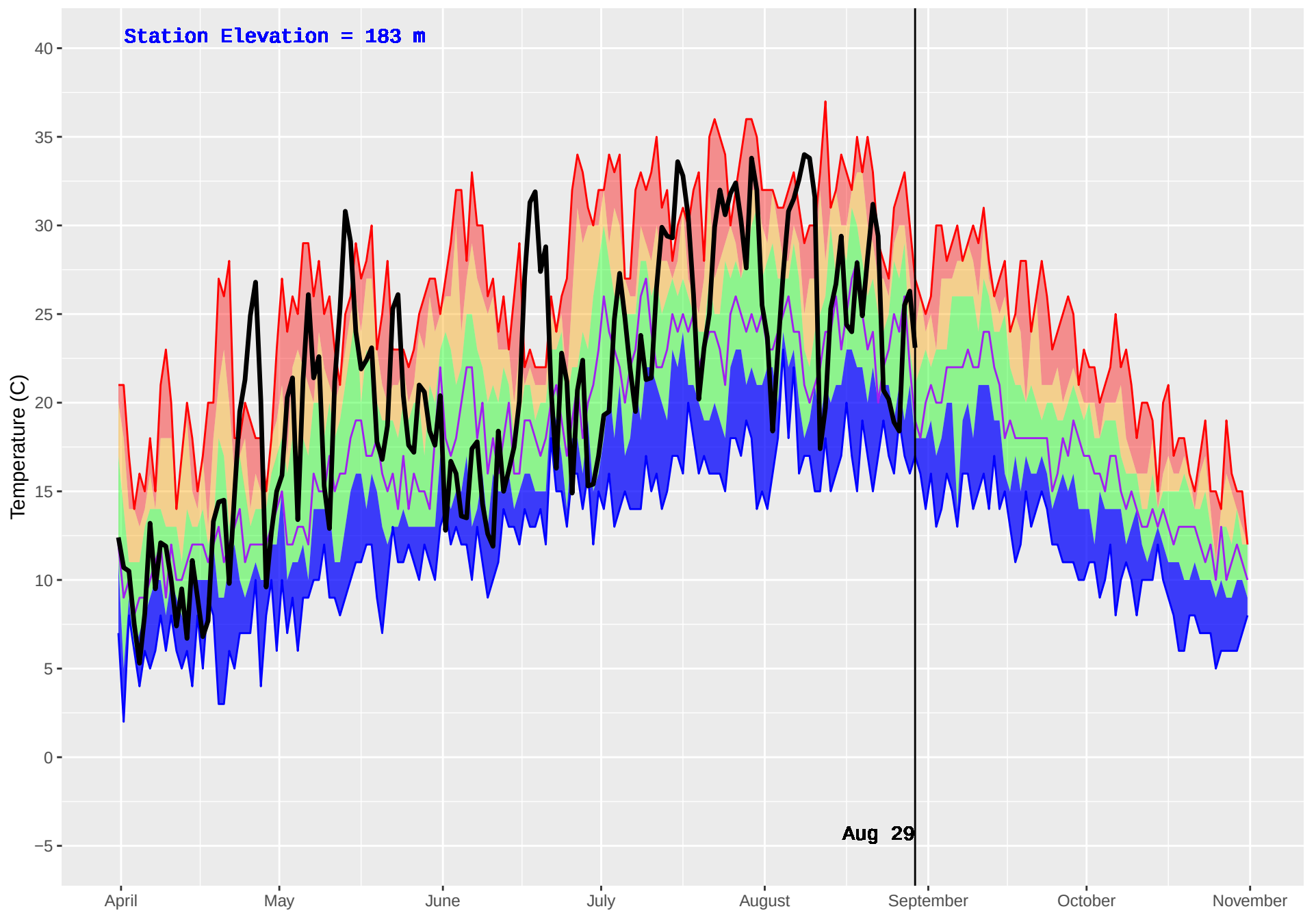
MESACHIE 2 (934) : Historical (2006–2016) and Current (2018) Daily Temperature
